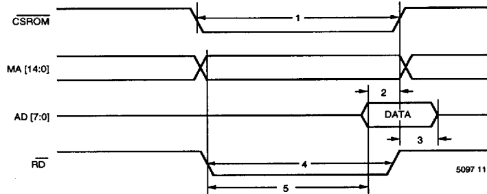
Figure 9a. External Program Storage Read Bus Cycle
