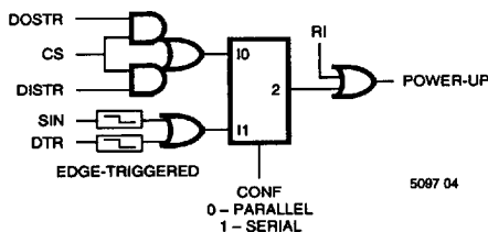
Figure 3. VALID Power-up Inputs
