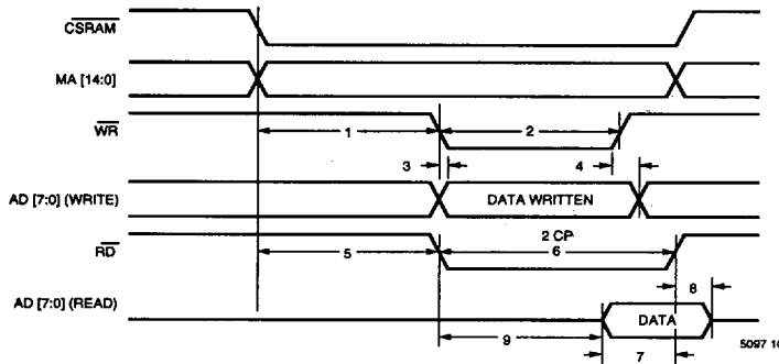
Figure 7. Oscillator, Internal (+2) Clock and CKOUT Timing
