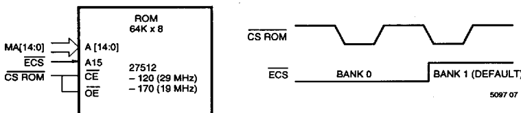
Figure 6a. OE Could be Grounded, But Above Connection Saves Power in PD Mode.
