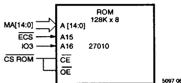
Figure 6b. 128K ROM Connections
