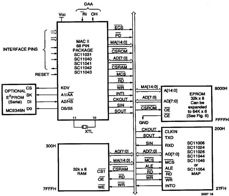
Figure 16. MAC II 68 Pin Package Interfaces to Serial E 2 PROM, ROM Map for Serial Interface Configurations
