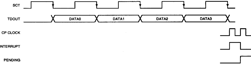
Figure 4. TX Timing Diagram
